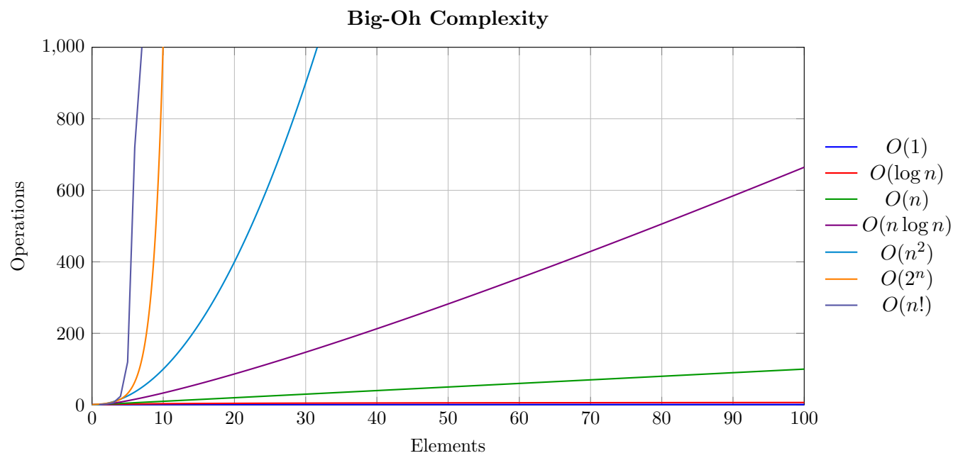
Figure 4.1: Common Big-Oh growth rates. Graph recreated from the visual included in cletus, “What is a plain English explanation of ‘Big O’ notation?,” Stack Overflow , https://stackoverflow.com/questions/487258/what-is-a-plain-english-explanation-of-big-o-notation .
